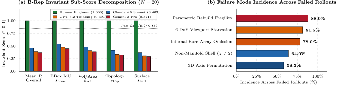
Figure 2: Empirical evaluation on the 20-task spacetime-ml/cad-cua benchmark. (a) Mean composite RLVR reward R and sub-score breakdown ( \bar{s}_{\text{bbox}} , \bar{s}_{\text{vol}} , \bar{s}_{\text{top}} , \bar{s}_{\text{surf}} ) across human ground truth and frontier models. (b) Incidence of the five primary 3D CAD failure modes across failed frontier model rollouts.
